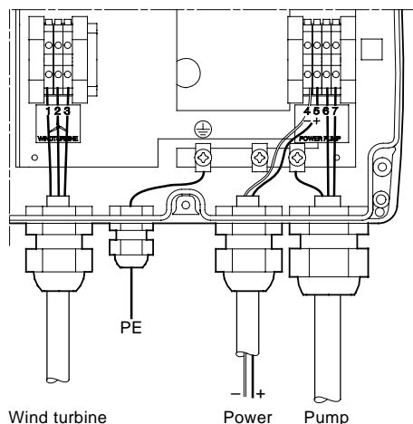
Fig. 25 Electrical connections
