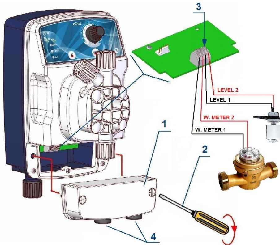
Fig. 10 – Level probe connection
